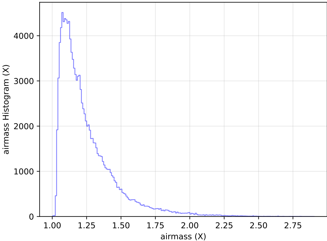
too_elab_r8_d3_ugrizy_v3.4_10yrs All sky u band: airmass Histogram
