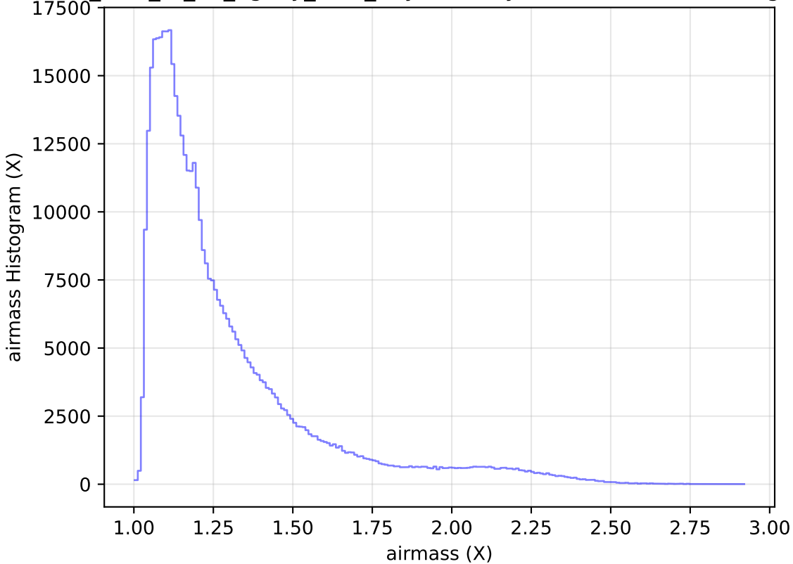
too_elab_r8_d3_ugrizy_v3.4_10yrs All sky r band: airmass Histogram
