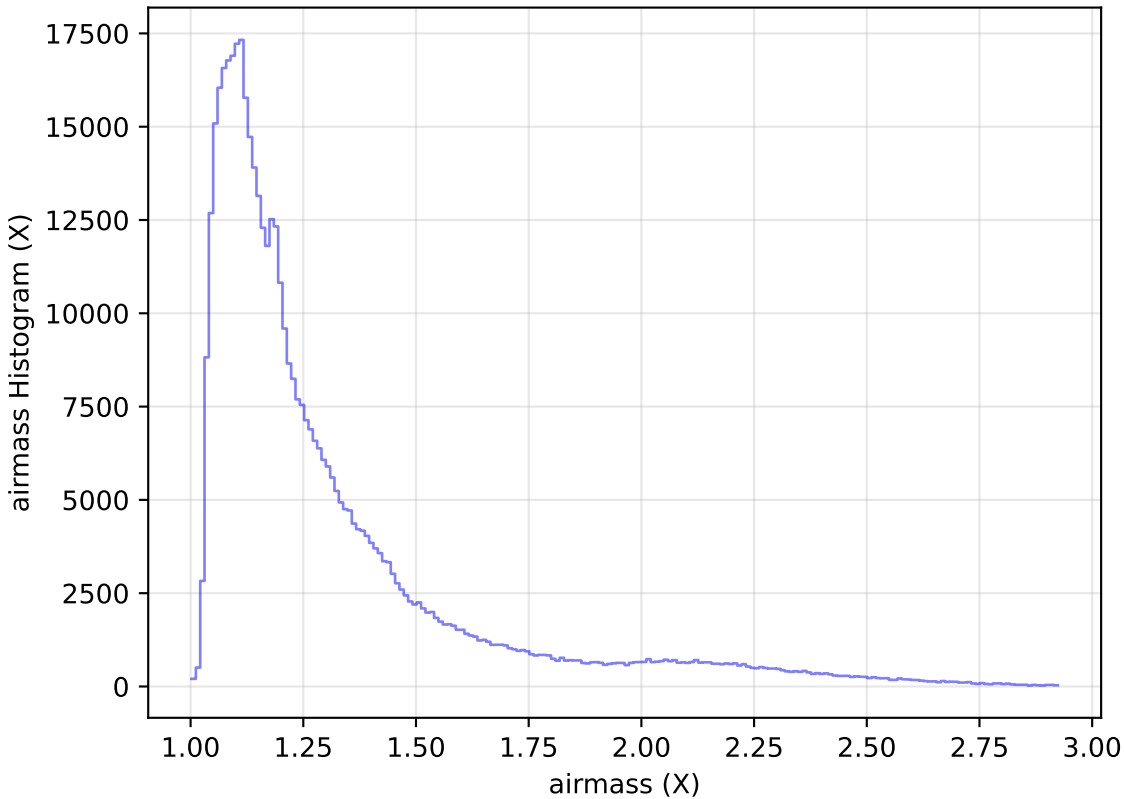
too_elab_r8_d3_ugrizy_v3.4_10yrs All sky i band: airmass Histogram
