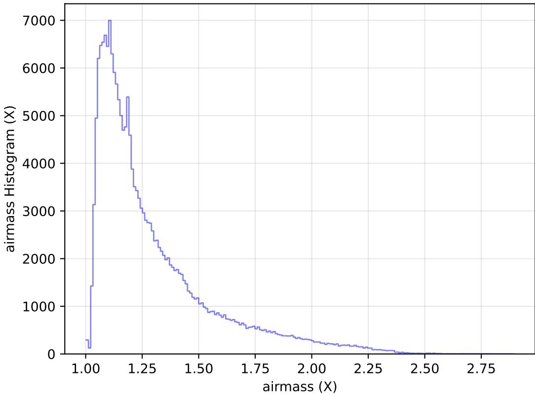
too_elab_r8_d3_ugrizy_v3.4_10yrs All sky g band: airmass Histogram
