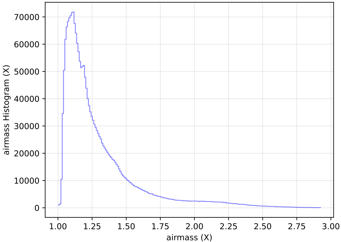
too_elab_r8_d3_ugrizy_v3.4_10yrs All sky all bands: airmass Histogram
