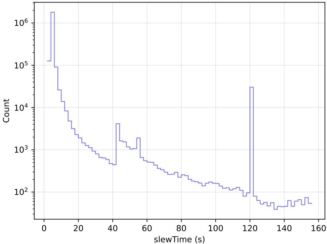
too_elab_r8_d3_ugrizy_v3.4_10yrs All visits: Slew Time Histogram
