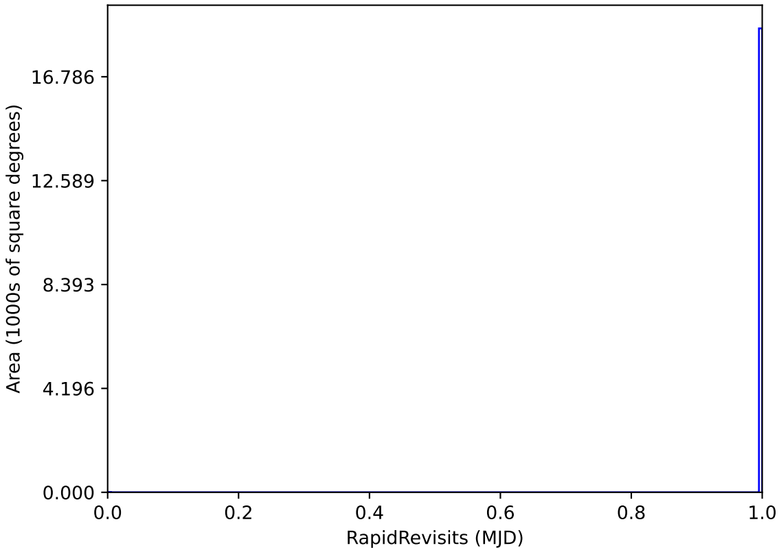
too_elab_r8_d3_ugrizy_v3.4_10yrs WFD: RapidRevisits
