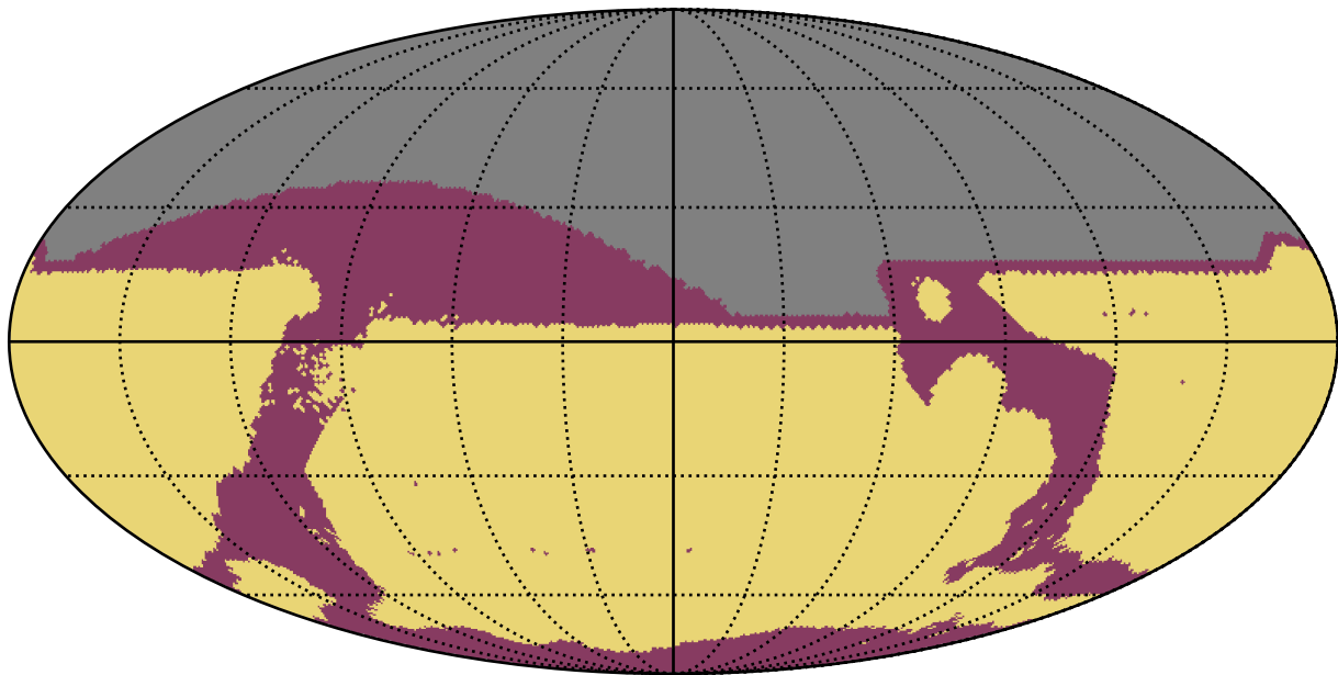
too_elab_r8_d3_ugrizy_v3.4_10yrs All sky: RapidRevisits
