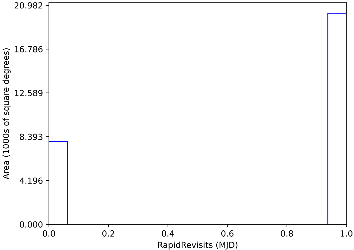
too_elab_r8_d3_ugrizy_v3.4_10yrs All sky: RapidRevisits
