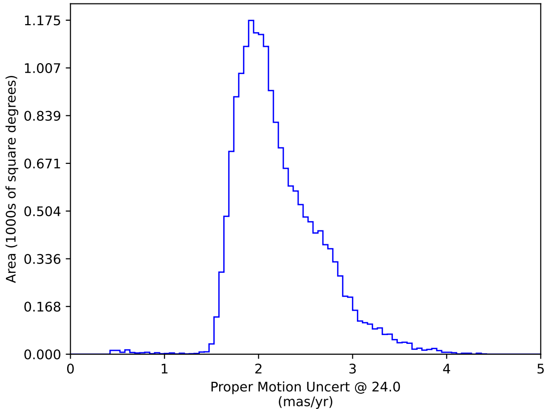
too_elab_r8_d3_ugrizy_v3.4_10yrs WFD: Proper Motion Uncert @ 24.0
