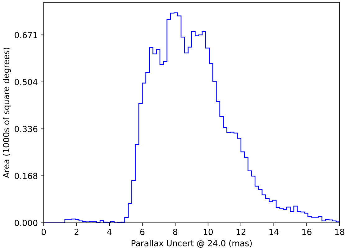
too_elab_r8_d3_ugrizy_v3.4_10yrs WFD: Parallax Uncert @ 24.0
