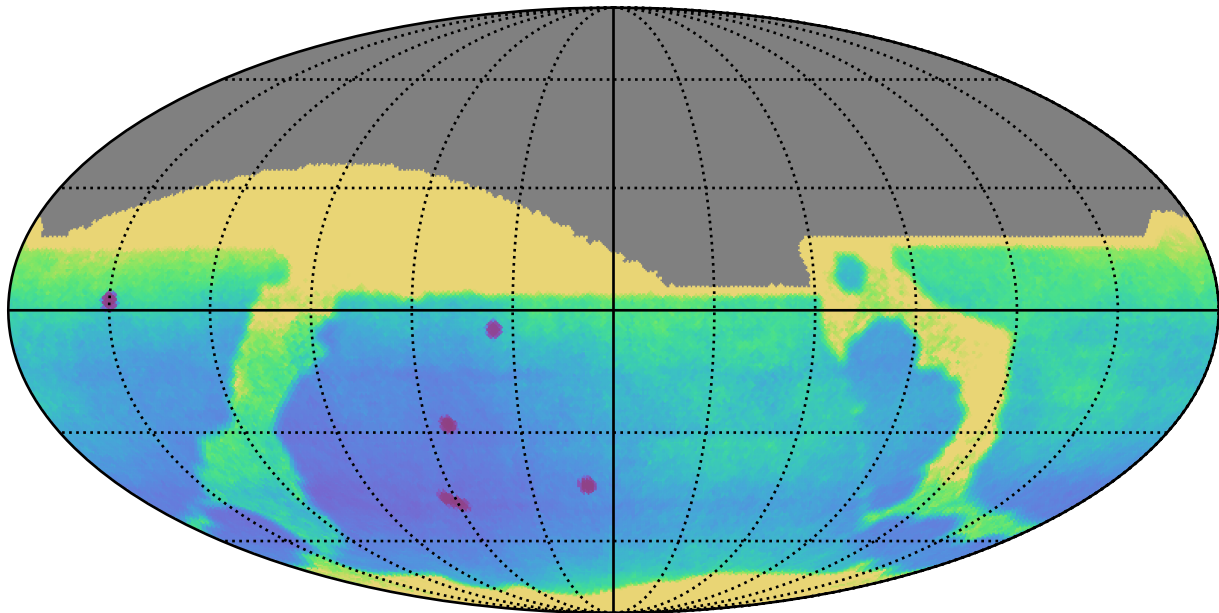
too_elab_r8_d3_ugrizy_v3.4_10yrs All sky: Parallax Uncert @ 24.0
