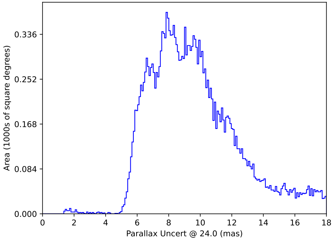
too_elab_r8_d3_ugrizy_v3.4_10yrs All sky: Parallax Uncert @ 24.0
