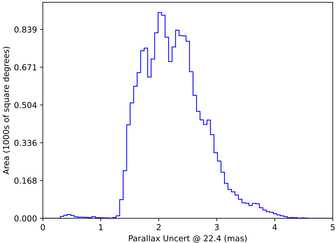
too_elab_r8_d3_ugrizy_v3.4_10yrs WFD: Parallax Uncert @ 22.4
