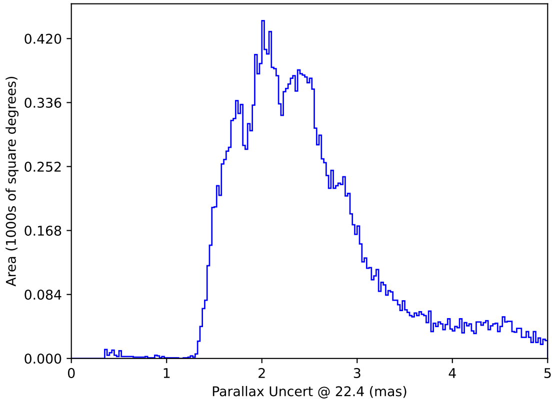
too_elab_r8_d3_ugrizy_v3.4_10yrs All sky: Parallax Uncert @ 22.4
