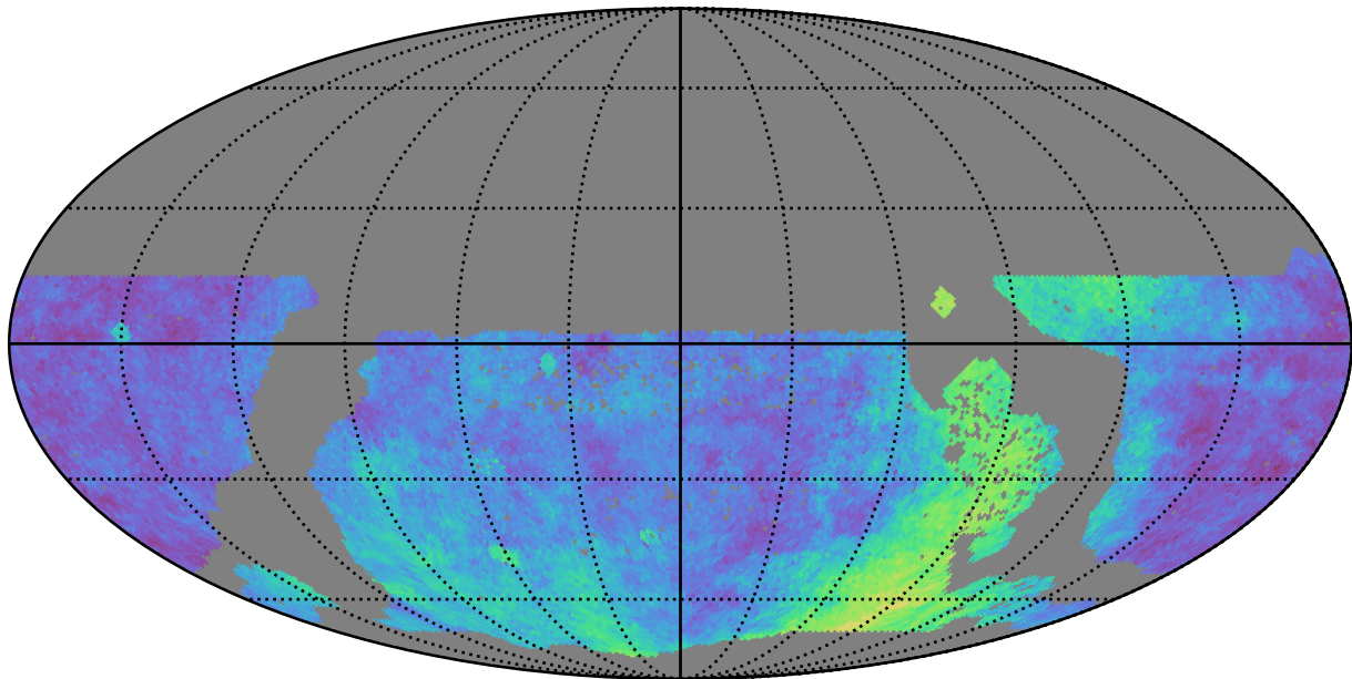
too_elab_r8_d3_ugrizy_v3.4_10yrs WFD: Parallax Coverage @ 24.0
