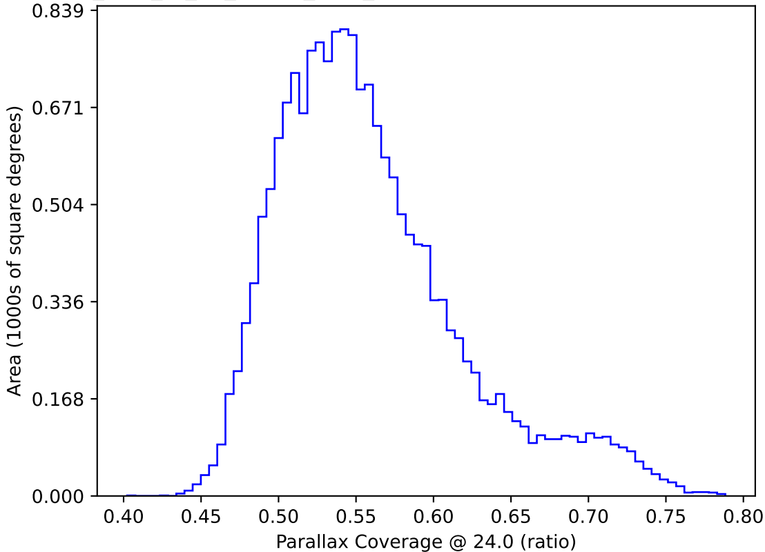
too_elab_r8_d3_ugrizy_v3.4_10yrs WFD: Parallax Coverage @ 24.0
