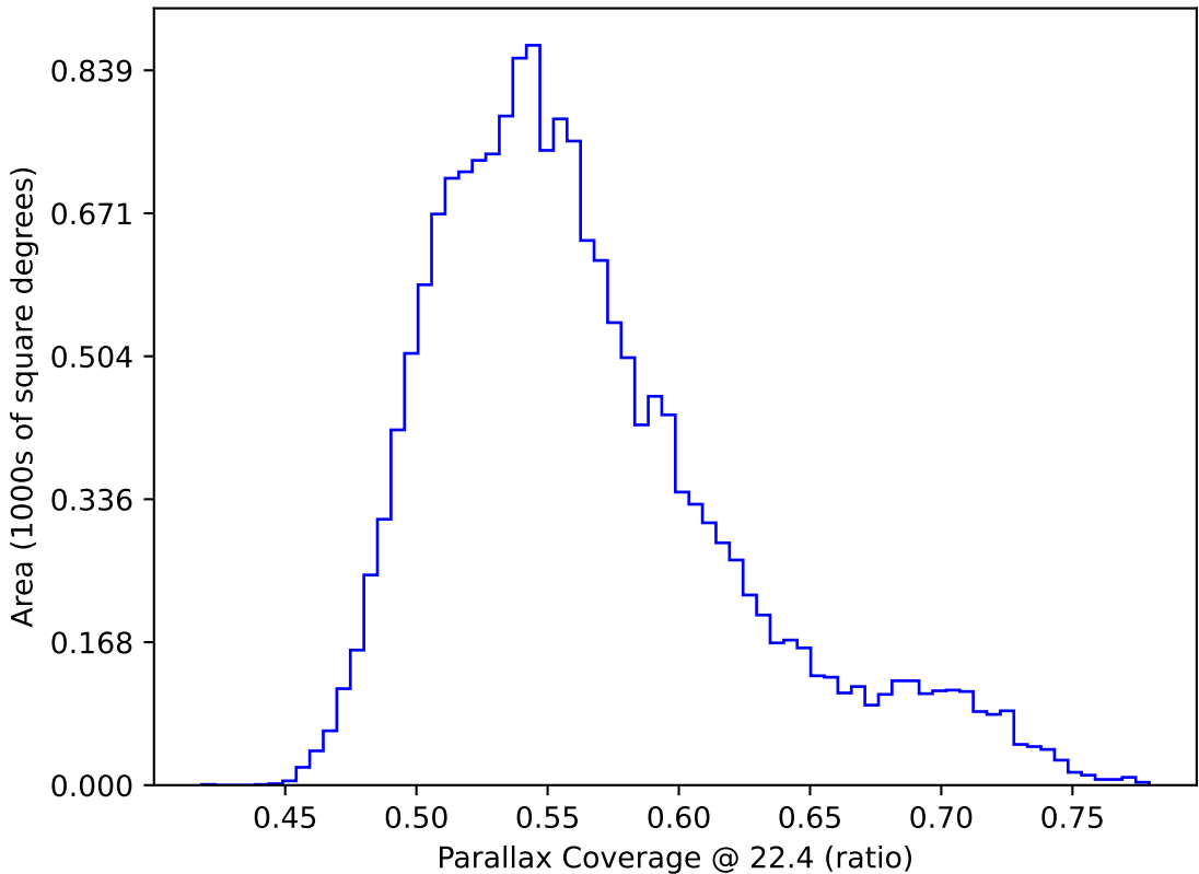
too_elab_r8_d3_ugrizy_v3.4_10yrs WFD: Parallax Coverage @ 22.4
