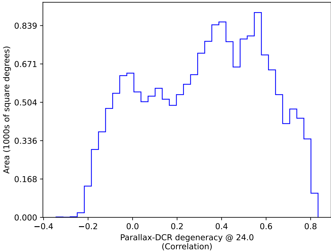
too_elab_r8_d3_ugrizy_v3.4_10yrs WFD: Parallax-DCR degeneracy @ 24.0
