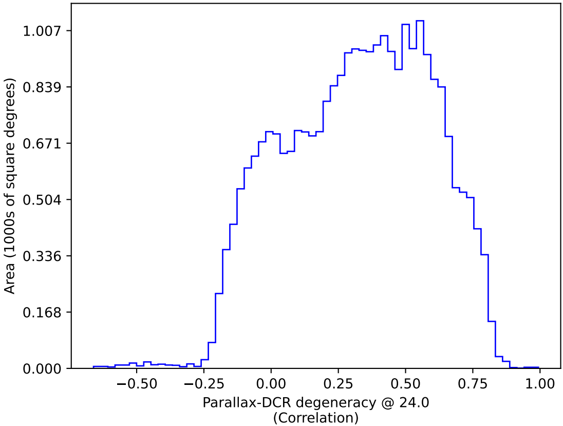
too_elab_r8_d3_ugrizy_v3.4_10yrs All sky: Parallax-DCR degeneracy @ 24.0
