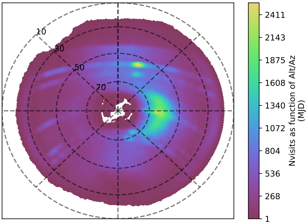
too_elab_r8_d3_ugrizy_v3.4_10yrs z band: Nvisits as function of Alt/Az
