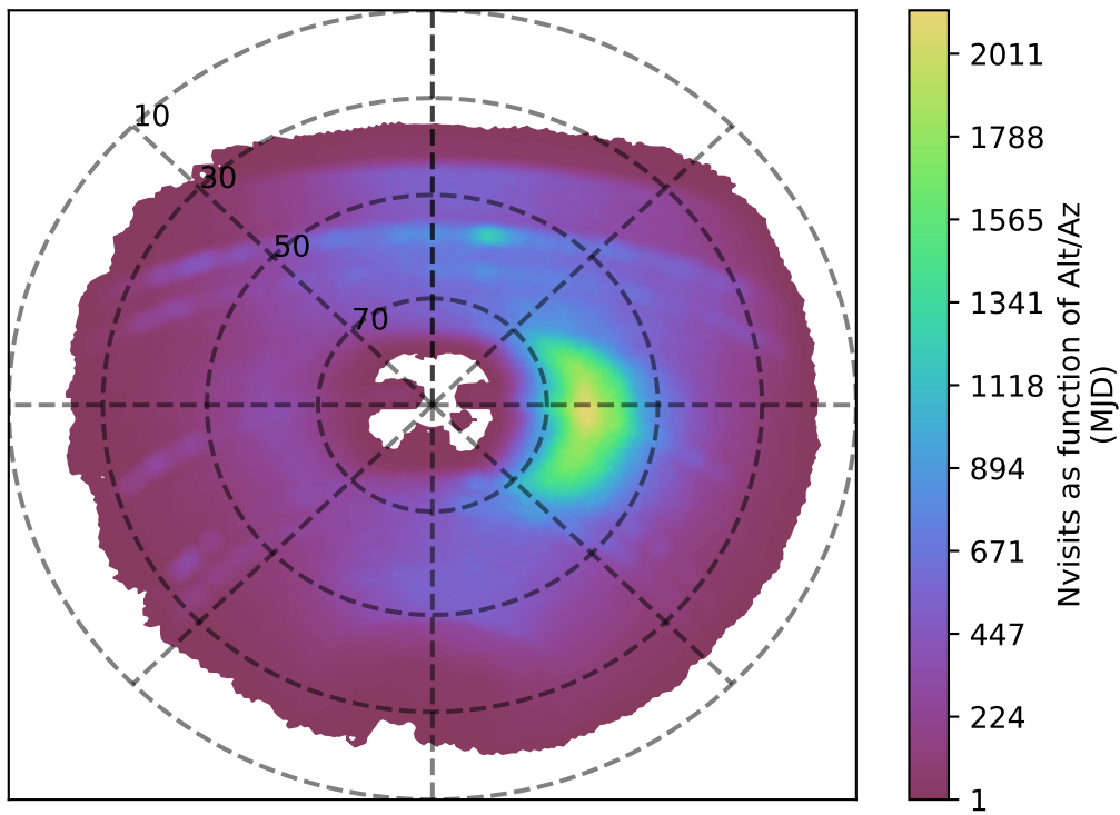
too_elab_r8_d3_ugrizy_v3.4_10yrs y band: Nvisits as function of Alt/Az
