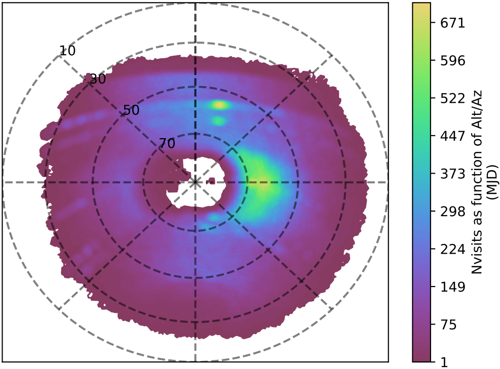
too_elab_r8_d3_ugrizy_v3.4_10yrs u band: Nvisits as function of Alt/Az
