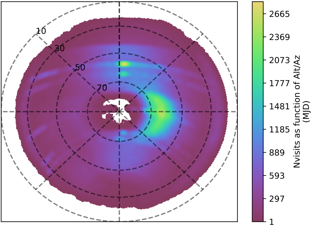
too_elab_r8_d3_ugrizy_v3.4_10yrs i band: Nvisits as function of Alt/Az
