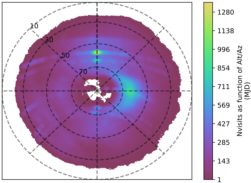
too_elab_r8_d3_ugrizy_v3.4_10yrs g band: Nvisits as function of Alt/Az
