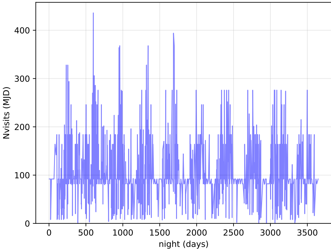
too_elab_r8_d3_ugrizy_v3.4_10yrs DDF: Nvisits
