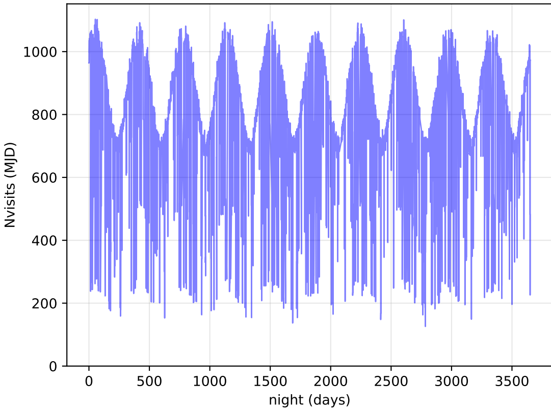
too_elab_r8_d3_ugrizy_v3.4_10yrs All visits: Nvisits
