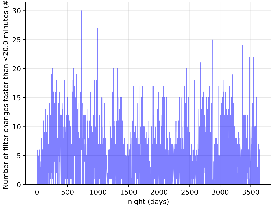
too_elab_r8_d3_ugrizy_v3.4_10yrs Per Night: Number of filter changes faster than <20.0 minutes
