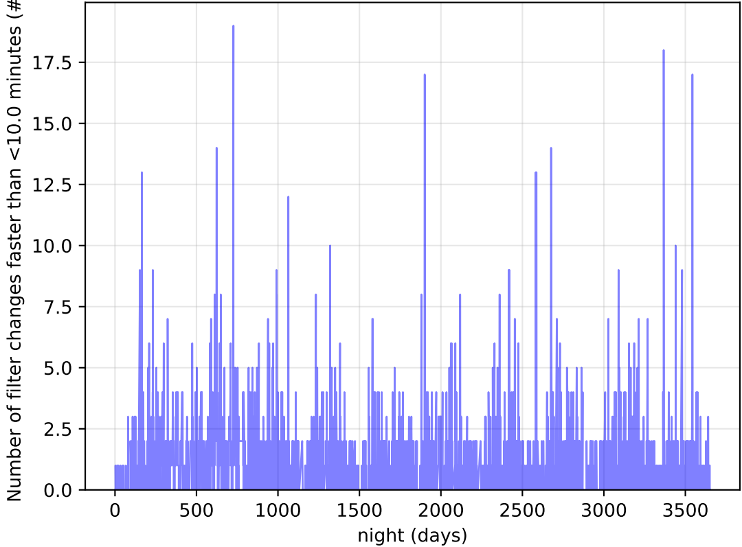
too_elab_r8_d3_ugrizy_v3.4_10yrs Per Night: Number of filter changes faster than <10.0 minutes
