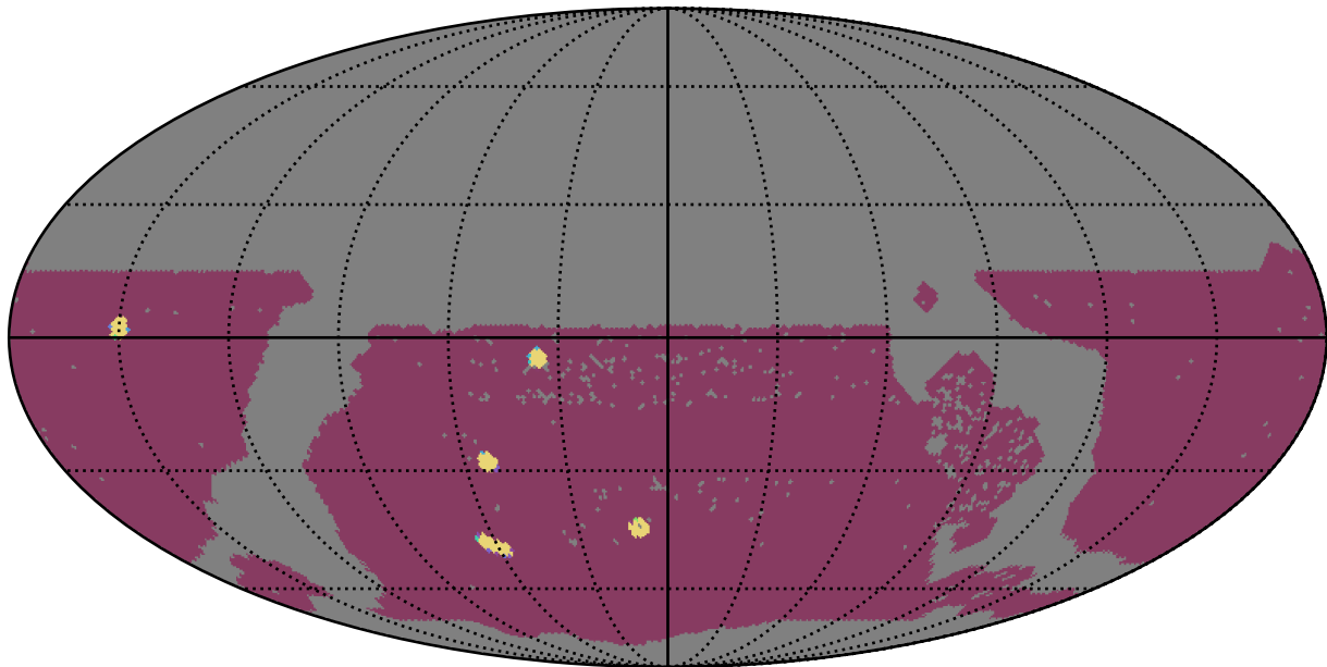
too_elab_r8_d3_ugrizy_v3.4_10yrs WFD: NumberOfQuickRevisits
