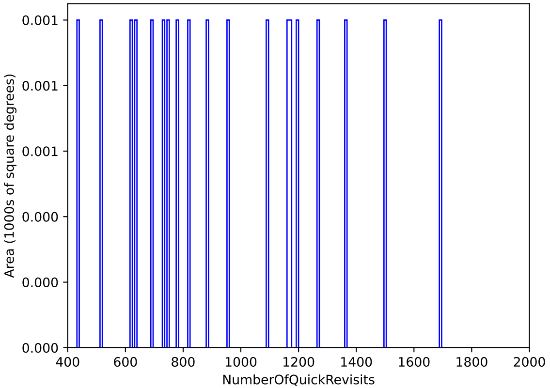
too_elab_r8_d3_ugrizy_v3.4_10yrs WFD: NumberOfQuickRevisits
