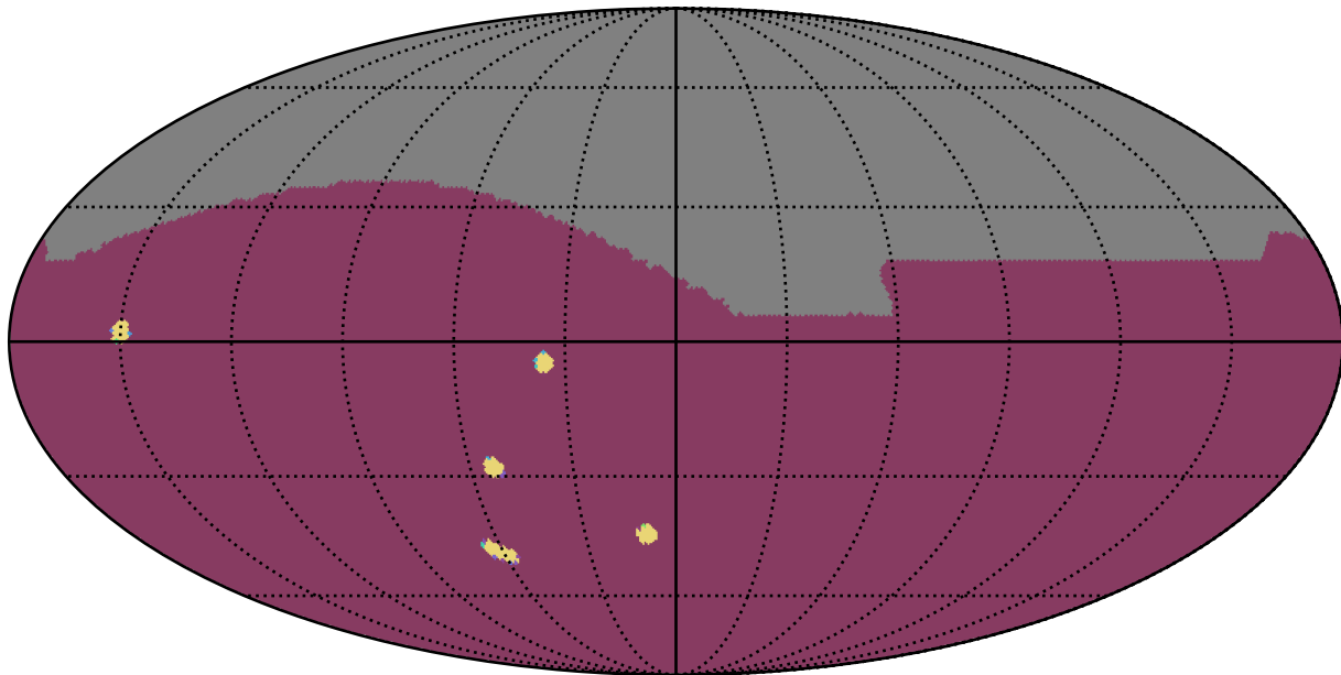
too_elab_r8_d3_ugrizy_v3.4_10yrs All sky: NumberOfQuickRevisits
