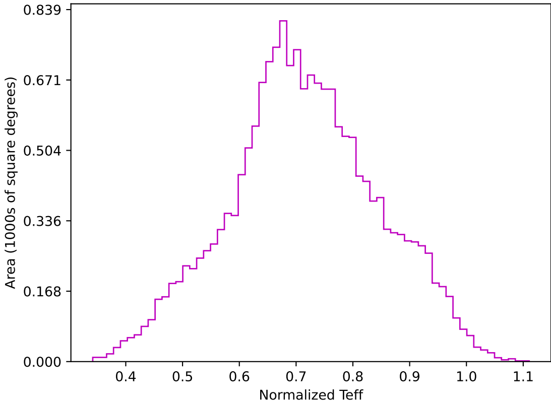
too_elab_r8_d3_ugrizy_v3.4_10yrs WFD z band: Normalized Teff
