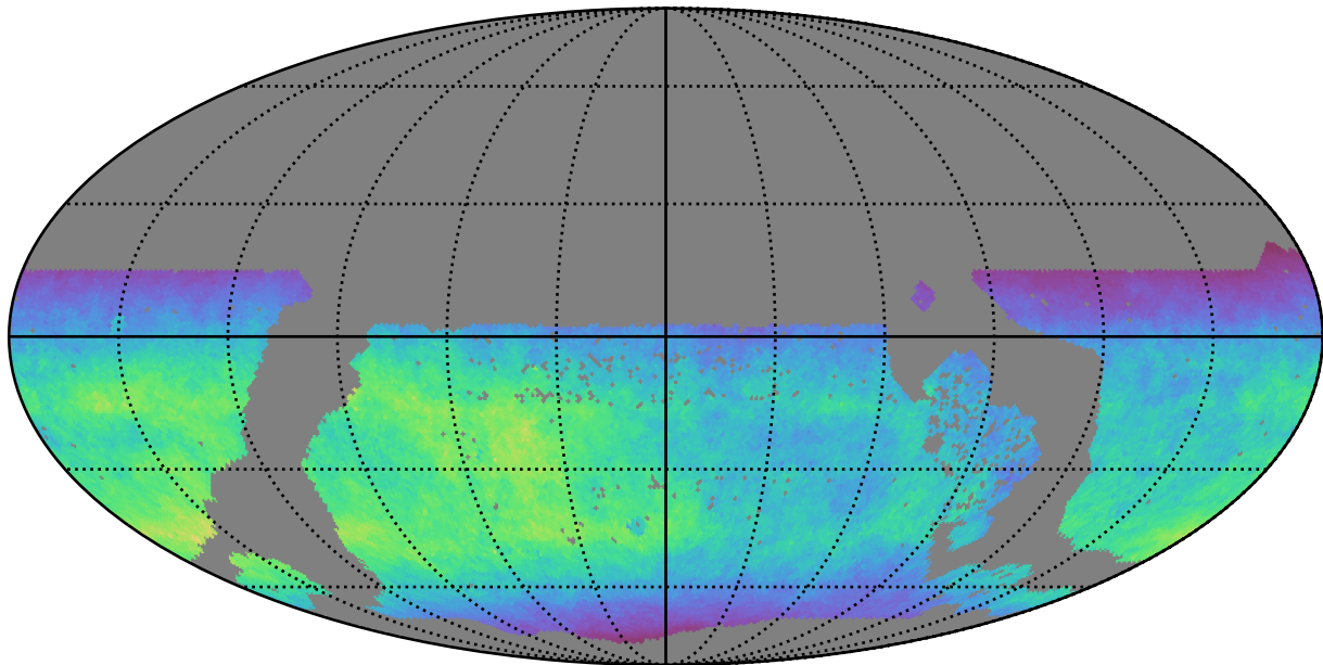
too_elab_r8_d3_ugrizy_v3.4_10yrs WFD y band: Normalized Teff
