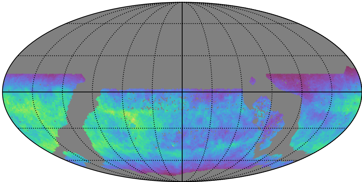
too_elab_r8_d3_ugrizy_v3.4_10yrs WFD u band: Normalized Teff
