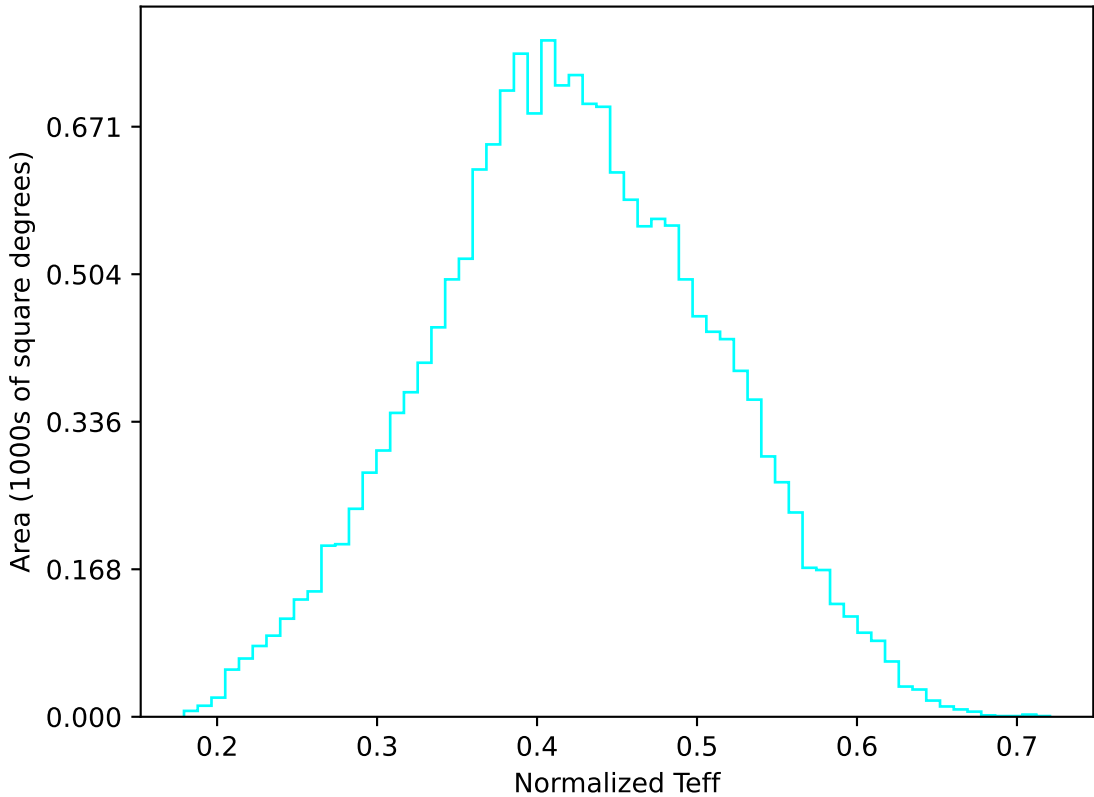
too_elab_r8_d3_ugrizy_v3.4_10yrs WFD u band: Normalized Teff
