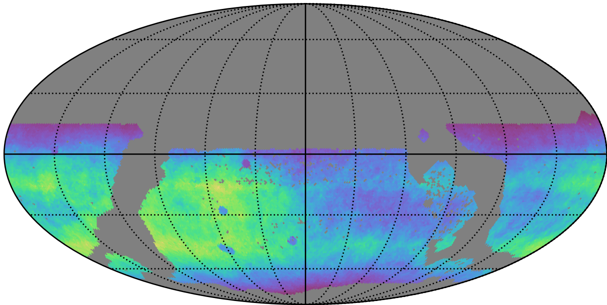
too_elab_r8_d3_ugrizy_v3.4_10yrs WFD r band: Normalized Teff
