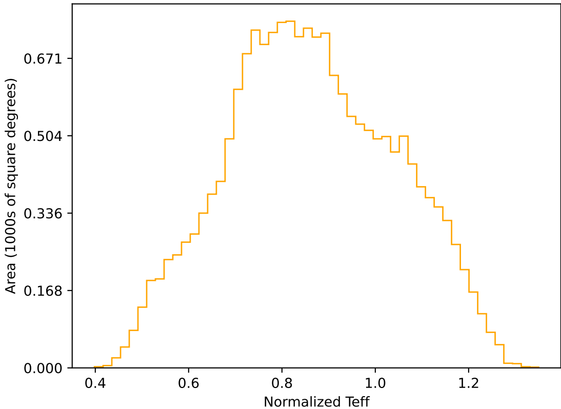
too_elab_r8_d3_ugrizy_v3.4_10yrs WFD r band: Normalized Teff
