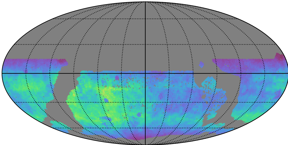
too_elab_r8_d3_ugrizy_v3.4_10yrs WFD g band: Normalized Teff
