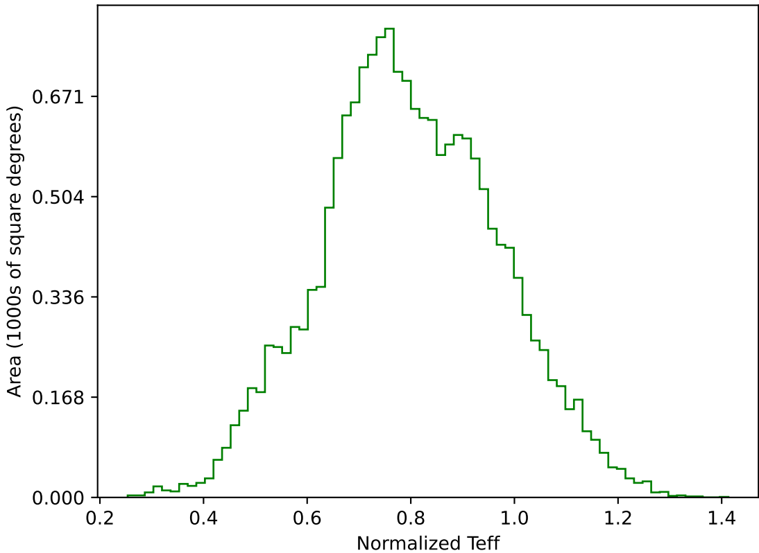
too_elab_r8_d3_ugrizy_v3.4_10yrs WFD g band: Normalized Teff
