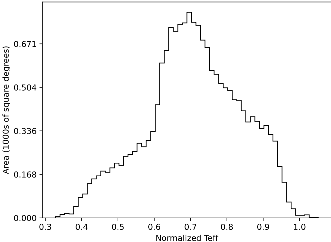
too_elab_r8_d3_ugrizy_v3.4_10yrs WFD all bands: Normalized Teff
