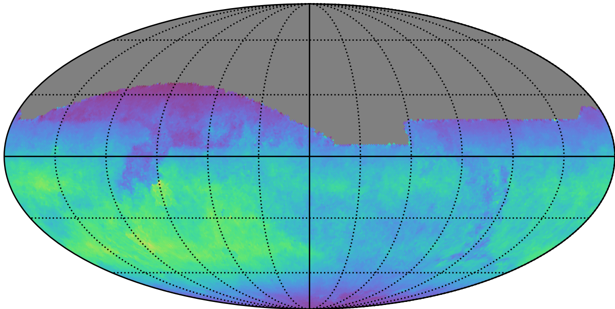
too_elab_r8_d3_ugrizy_v3.4_10yrs All sky z band: Normalized Teff
