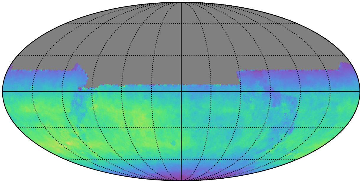
too_elab_r8_d3_ugrizy_v3.4_10yrs All sky y band: Normalized Teff
