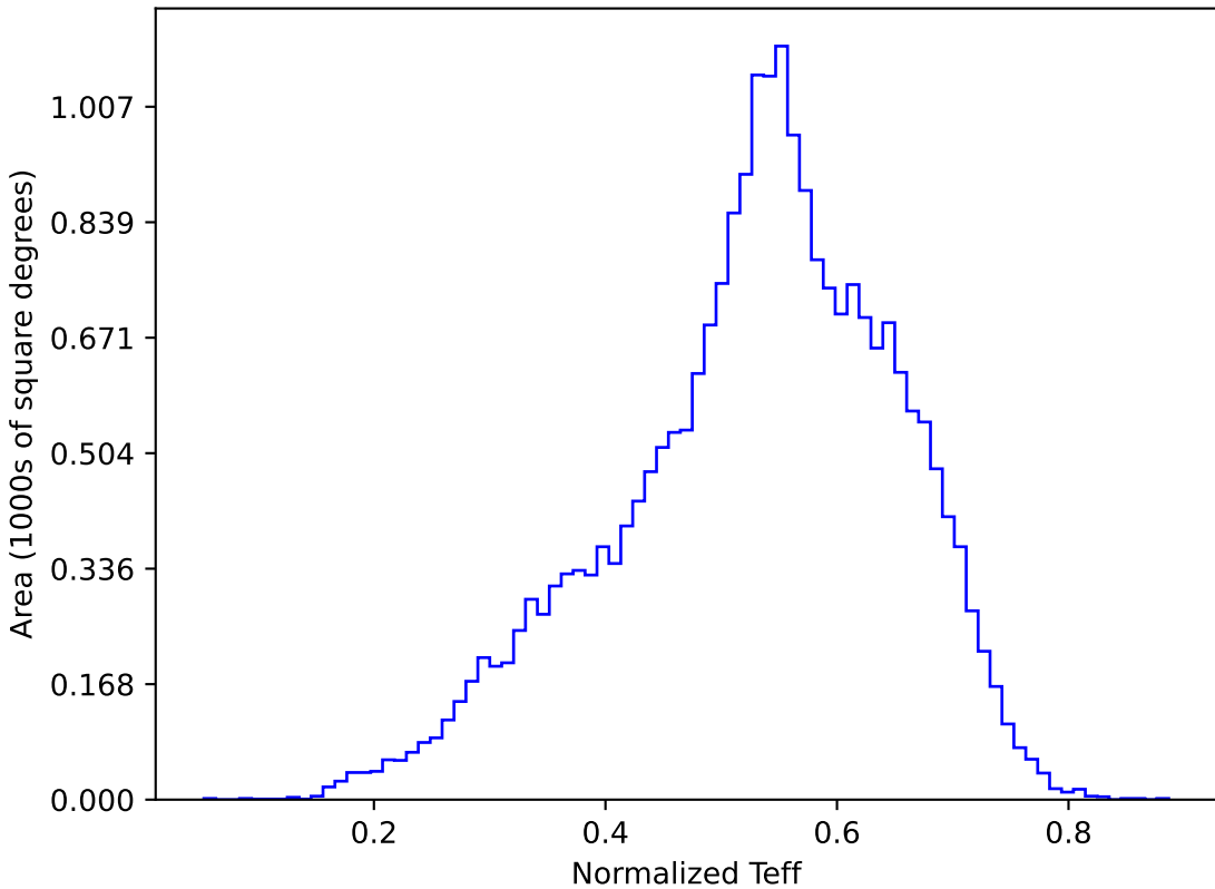
too_elab_r8_d3_ugrizy_v3.4_10yrs All sky y band: Normalized Teff
