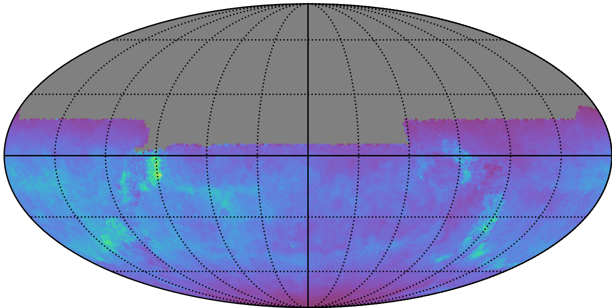
too_elab_r8_d3_ugrizy_v3.4_10yrs All sky u band: Normalized Teff
