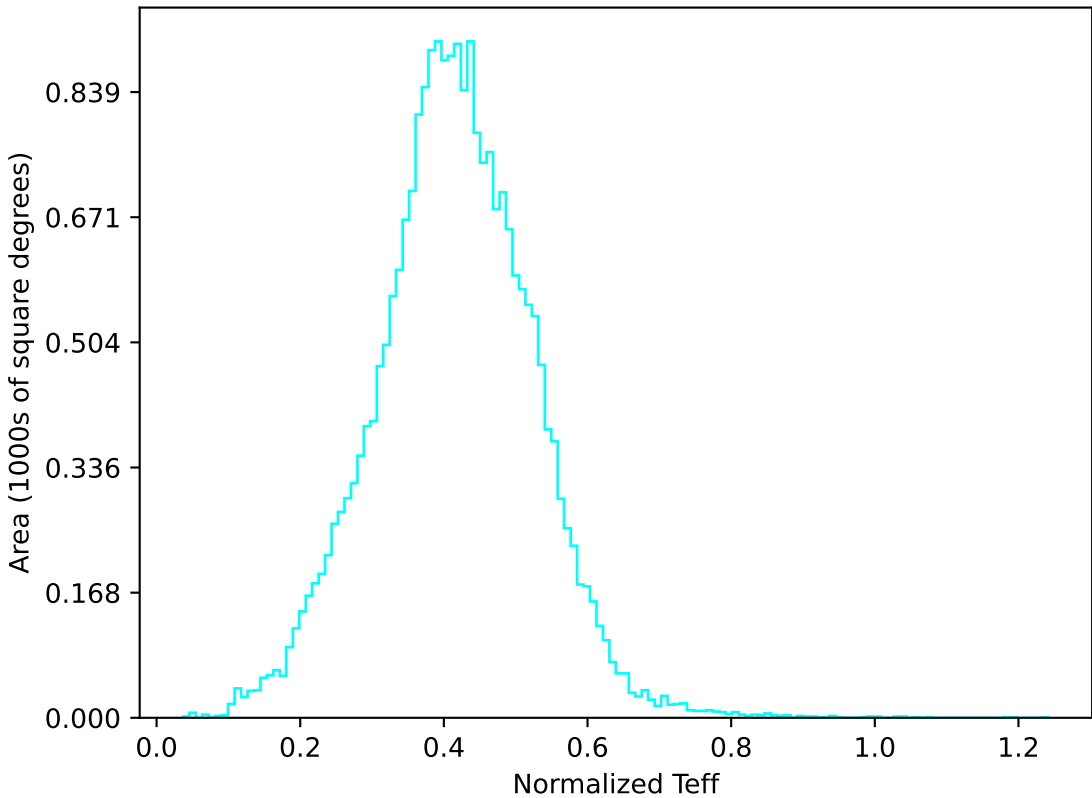
too_elab_r8_d3_ugrizy_v3.4_10yrs All sky u band: Normalized Teff
