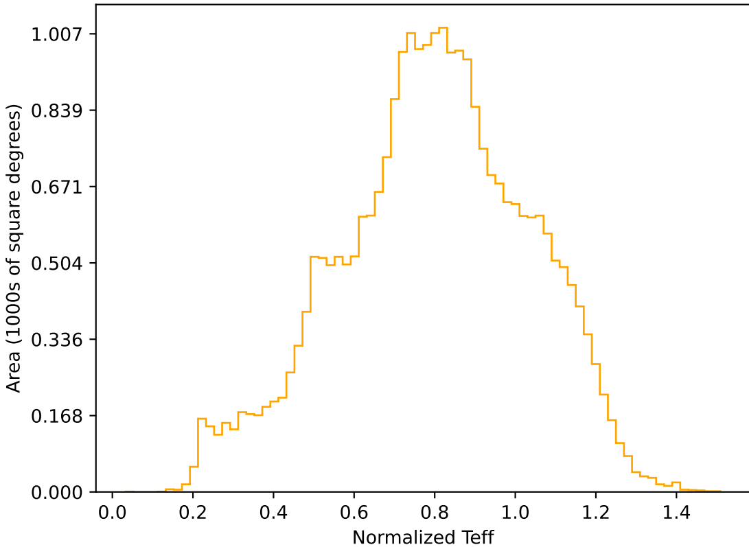
too_elab_r8_d3_ugrizy_v3.4_10yrs All sky r band: Normalized Teff
