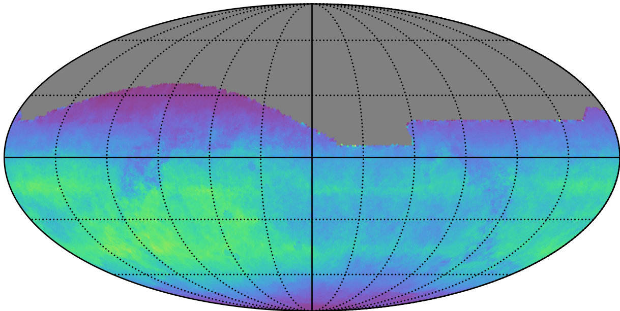
too_elab_r8_d3_ugrizy_v3.4_10yrs All sky i band: Normalized Teff
