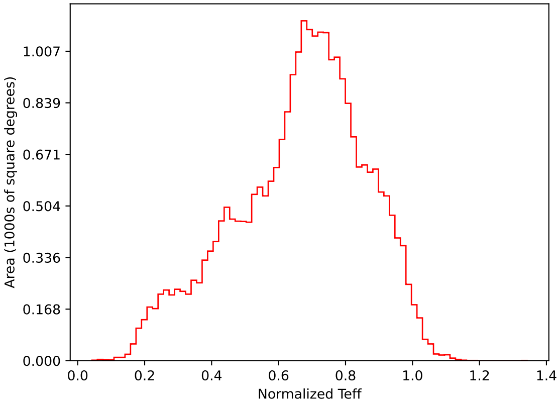
too_elab_r8_d3_ugrizy_v3.4_10yrs All sky i band: Normalized Teff
