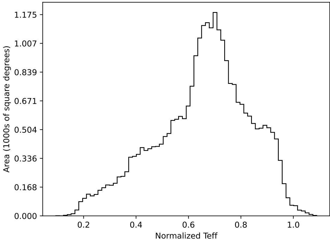
too_elab_r8_d3_ugrizy_v3.4_10yrs All sky all bands: Normalized Teff
